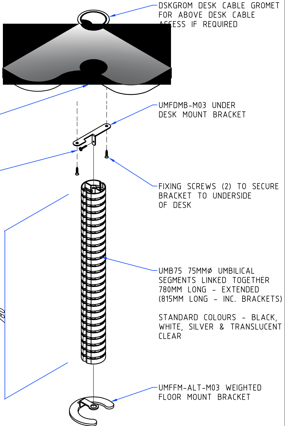
EXPLODED VIEW
