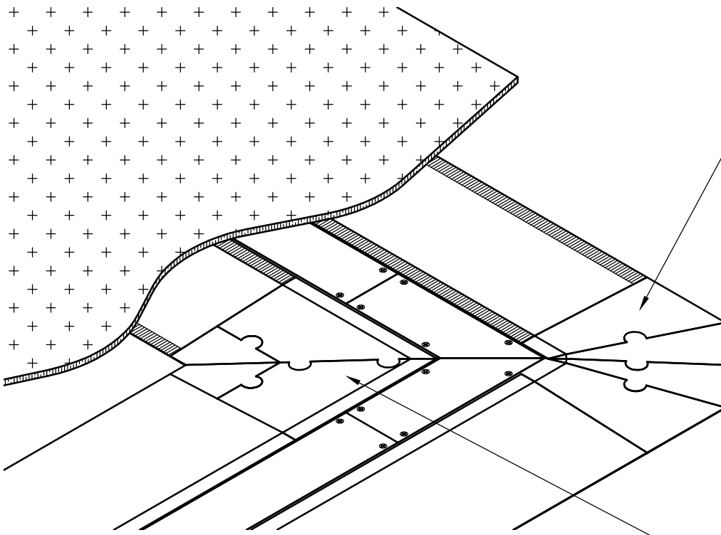
ASSEMBLED EXTERNAL BEND CARPET RAMP SECTION
