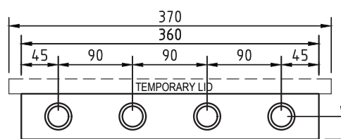
CONDUIT LOCATION OUTLET SIDES
