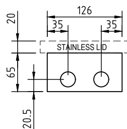
CONDUIT LOCATION SHORT (HINGE) SIDE
