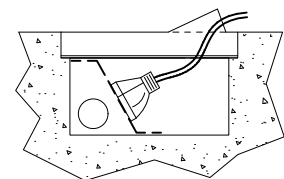
ASSEMBLED SIDE VIEW OF FB1SHD SINGLE COMPARTMENT FLOOR BOX SHOWING CABLE EXIT FLAP IN USE
