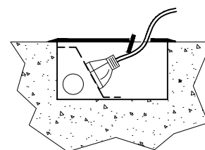
ASSEMBLED SIDE VIEW OF FB142 SINGLE COMPARTMENT FLOOR BOX SHOWING CABLE EXIT FLAP IN USE
