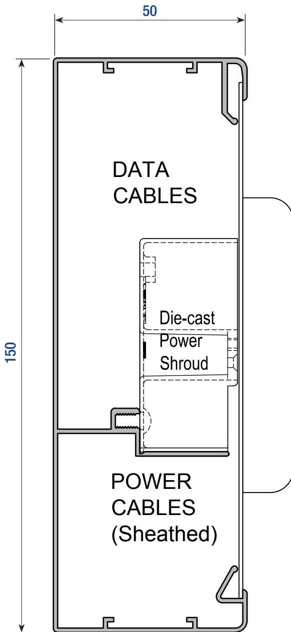
FULL SIZE SECTION
