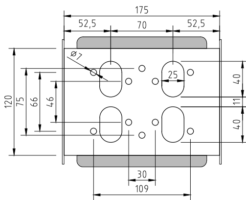
AFB70 CABLE ENTRY DETAILS
